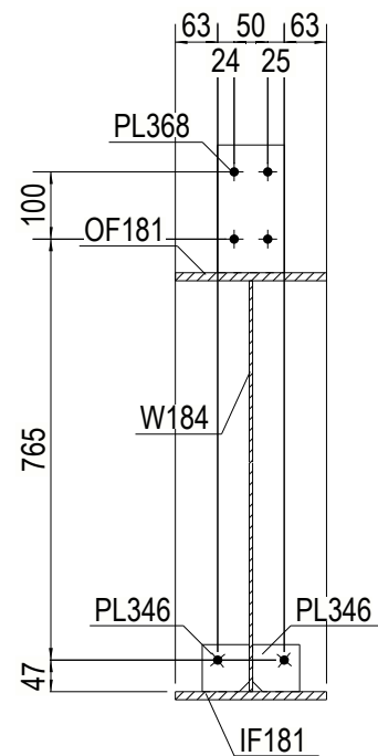
SEC A 1:12
