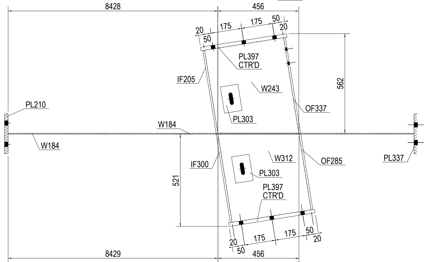
SEC B 1:12
